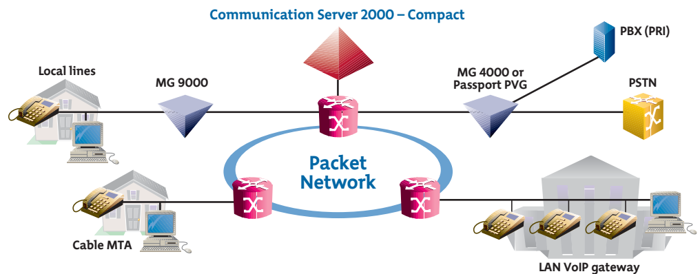
Figure 1. The packet-based Succession Communication Server 2000 – Compact supports traditional copper access, integrated access, and cable media applications as well as packet trunking solutions.
