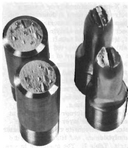
Fig. 2—Fracture appearance of smooth and notched tension-test specimens of maraging (250) steel showing longitudinal "splits" and "internal shear lips".
